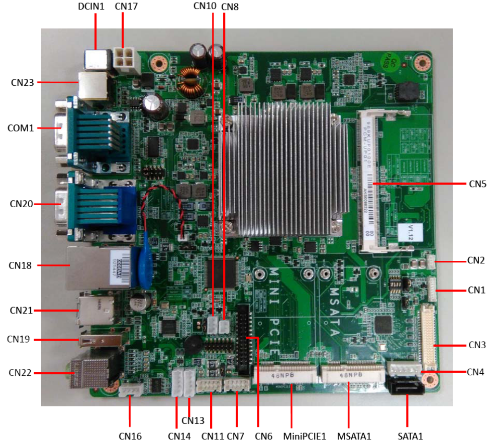
Figure 3.2 Connector Locations
