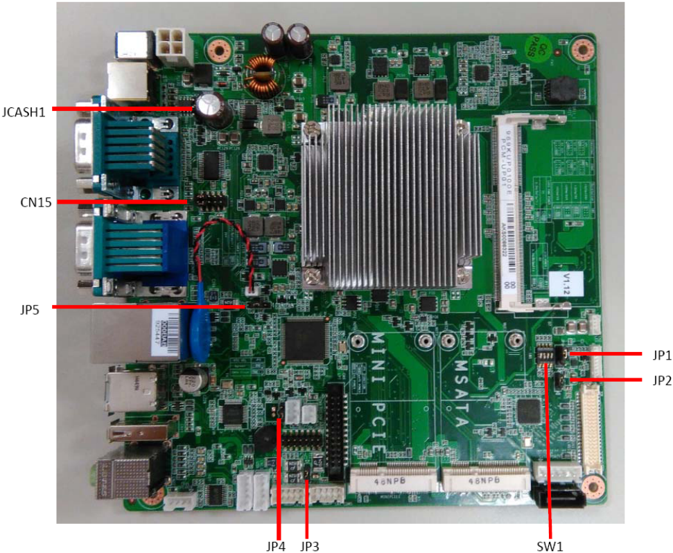
Figure 3.1 Jumper Locations
