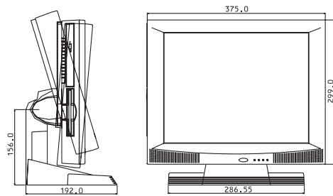
Desktop Stand (PPC-S155/S154)
