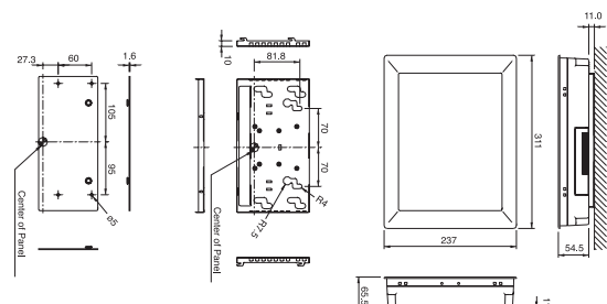
Wall Mount (PPC-S123)
