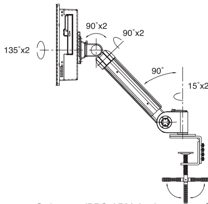
Swingarm (PPC-ARM-A03)
