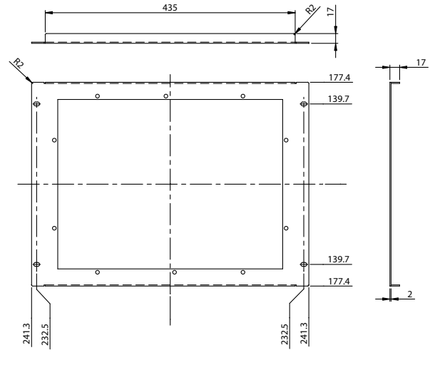
19" Rack plate (8U) for PPC-153/154
