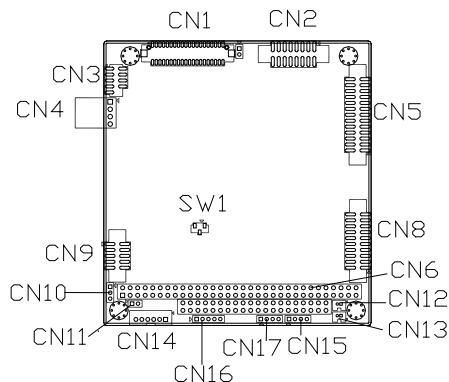
Figure1: PCM-3355 Location Connectors & Jumpers (component side)
