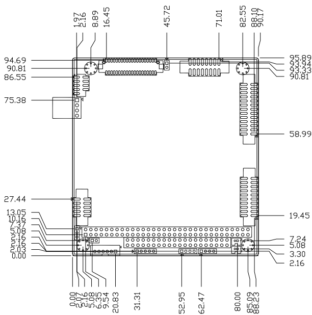
Figure 3: PCM-3355 Mechanical Drawing (component side)
