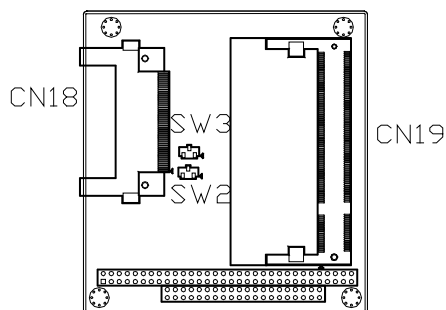
Figure2: PCM-3355 Location Connectors & Jumpers (solder side)
