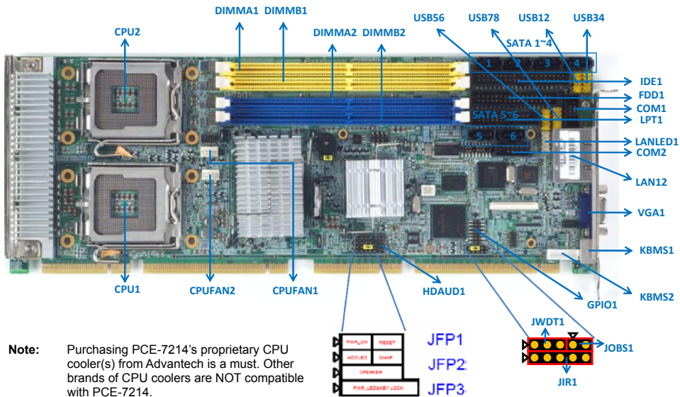
Board Layout: Jumper and Connector Location
