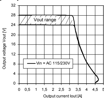
Output characteristic V_{out}/I_{out} (min.)
