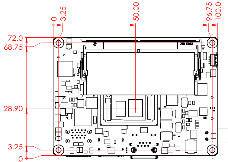
Figure 2.1 MIO-2364 Mechanical Drawing (Top Side)
