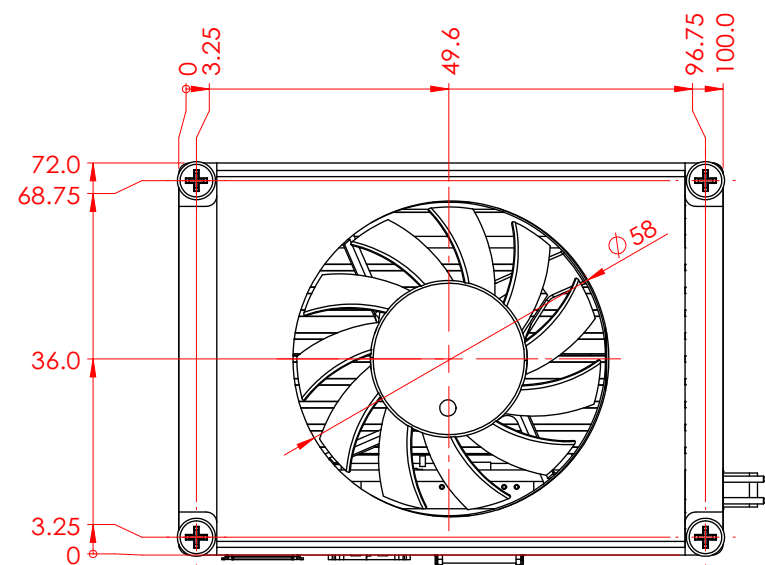
Figure 2.4 MIO-2364 Mechanical Drawing (with Cooler)
