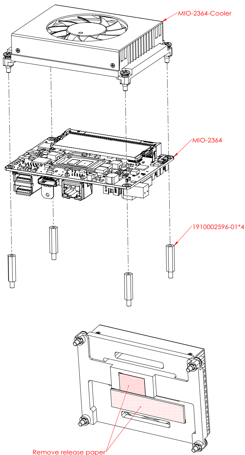
COOLER -MIO-2364-Remove release paper
