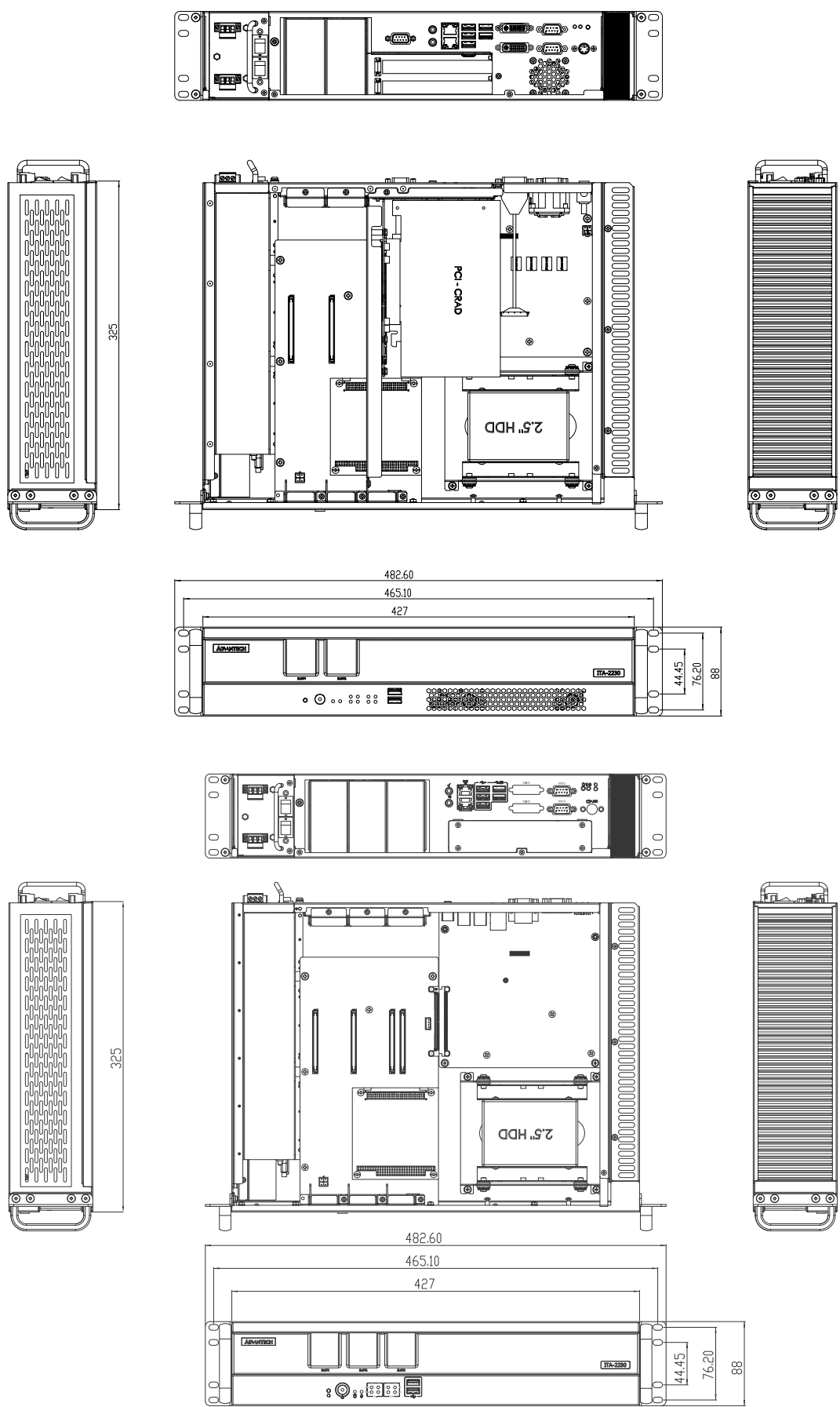
Figure 1.1 ITA-2230S Dimension
