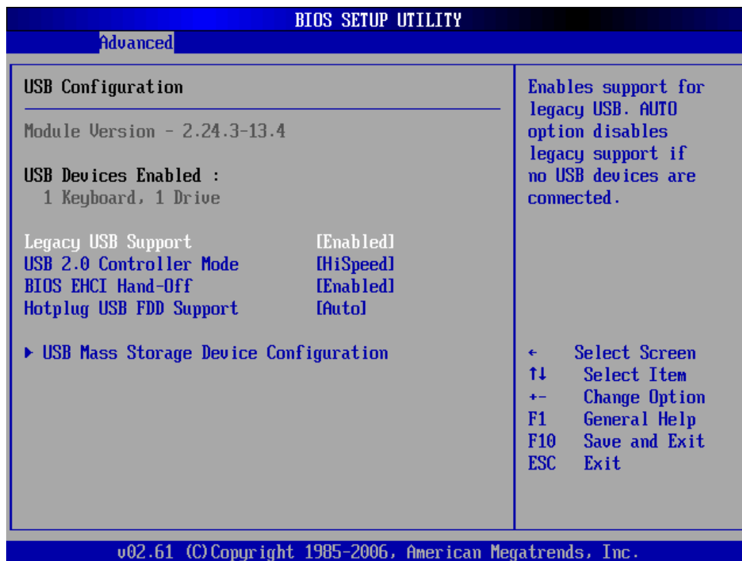
Figure 4.16: USB Configuration
