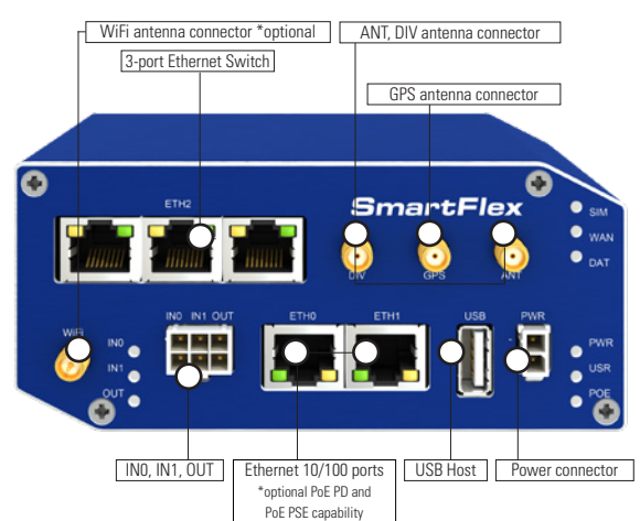
FRONT VIEW - BB-SR304xx4xx
