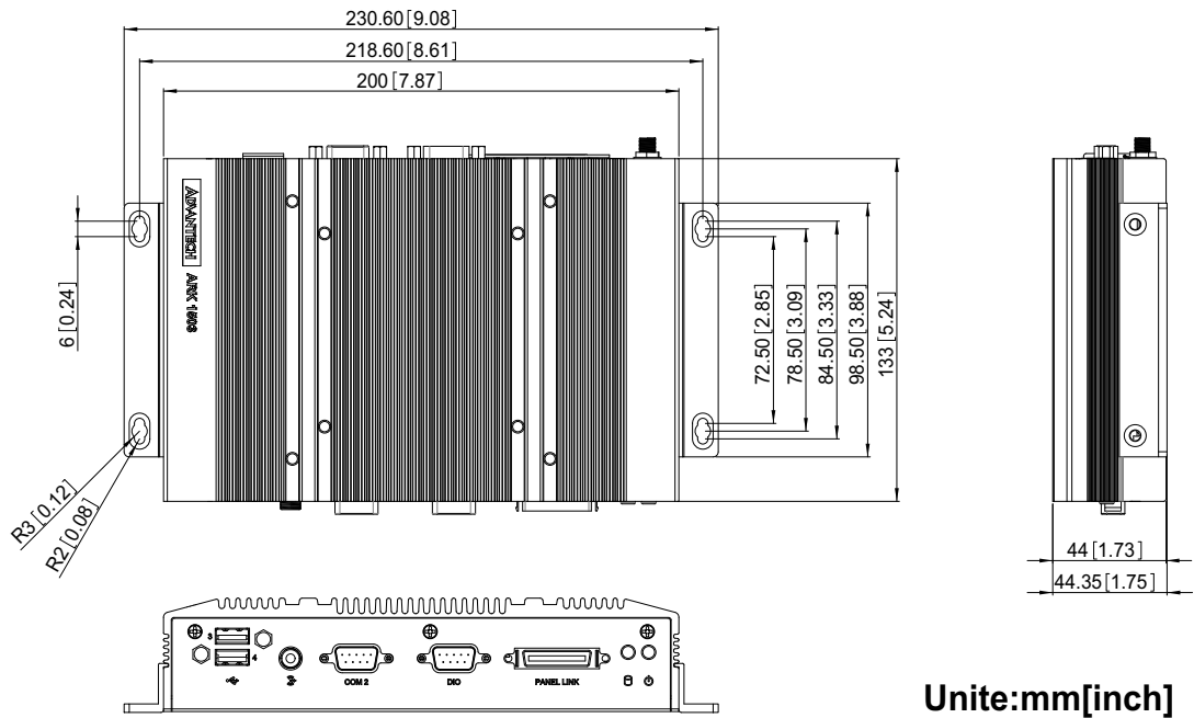
Figure 1.1 ARK-1503 Mechanical dimension drawing
