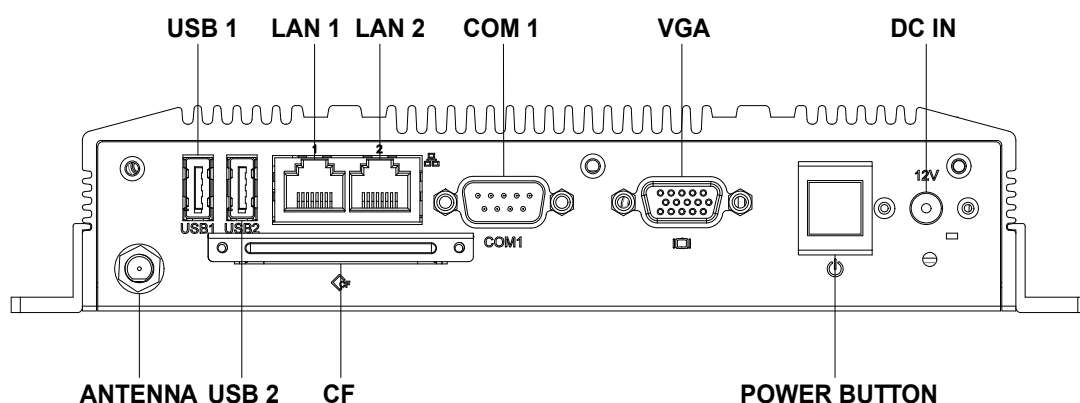
Figure 2.1 ARK-1503 Front View
