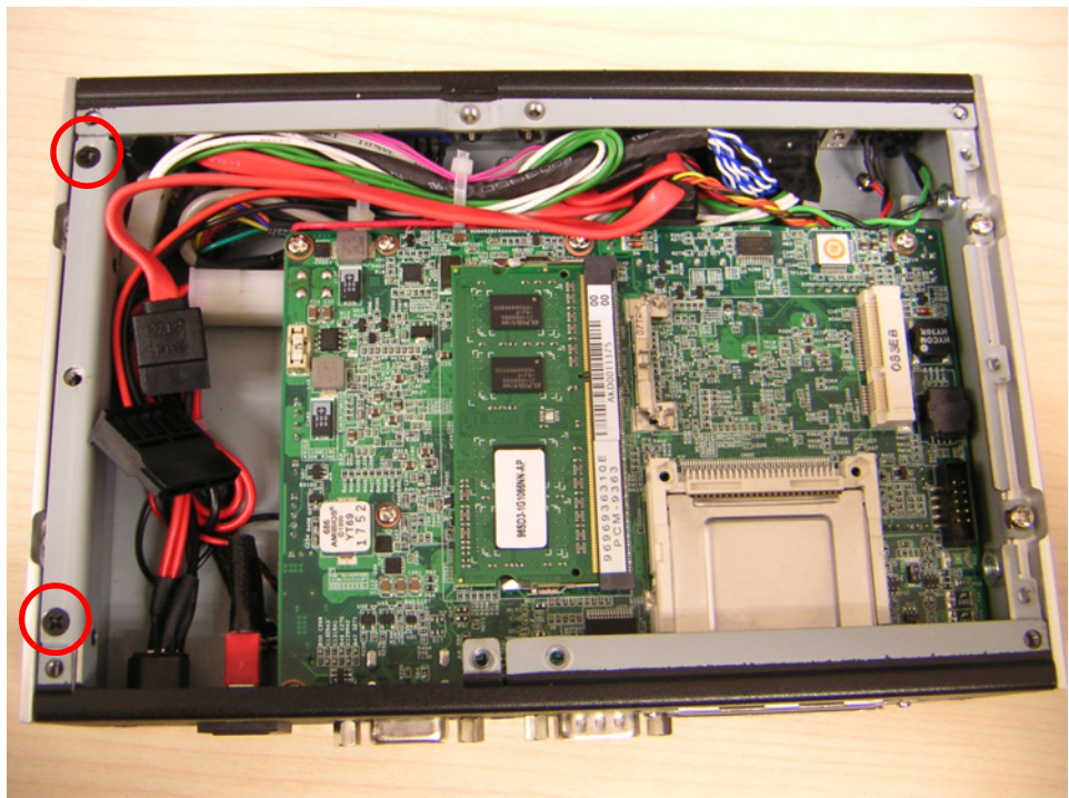
Figure 2.19 Unscrew the screws of the left HDD bracket
