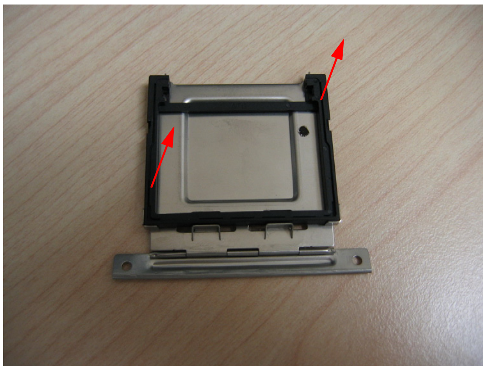
Figure 2.14 Remove the dummy CF bracket
