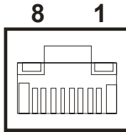
Figure 2.5 Ethernet Connector
