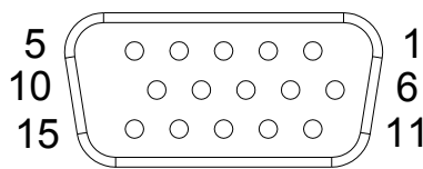
Figure 2.6 VGA Connector
