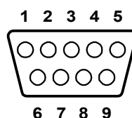
Figure 2.11 DIO Cable
