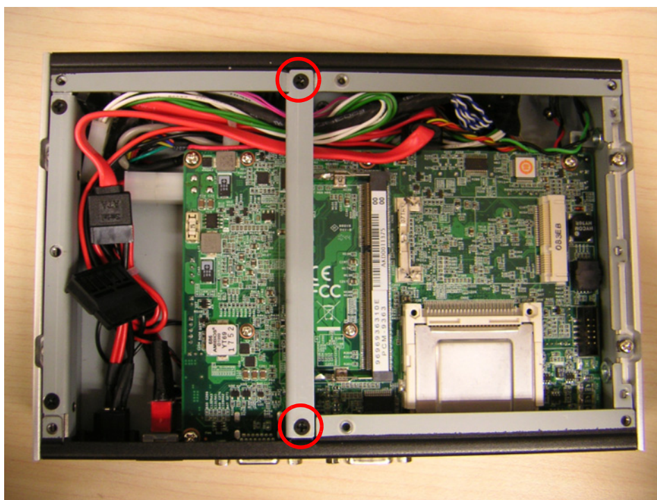
Figure 2.17 Unscrew the screws of the right HDD bracket
