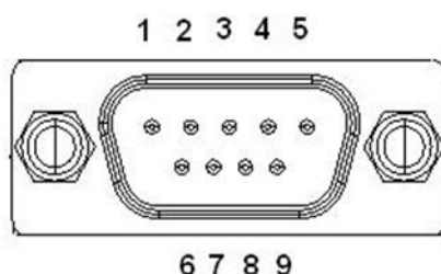
Figure 2.9 COM Port Connector
