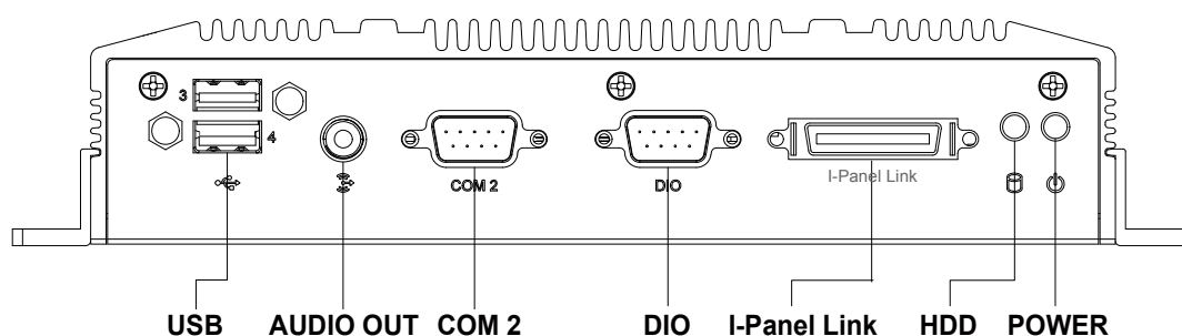
Figure 2.2 ARK-1503 Rear View
