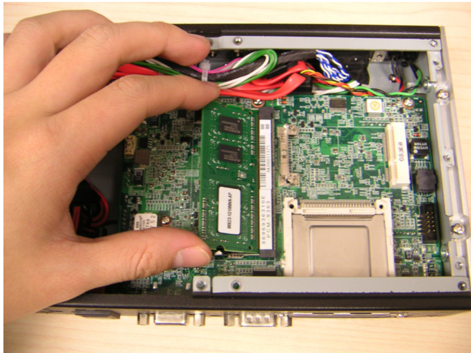
Figure 2.18 Install the RAM module
