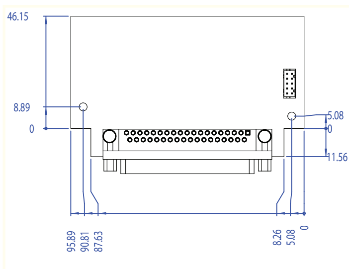
Figure 2: AIIS-DIO32 Dimension
