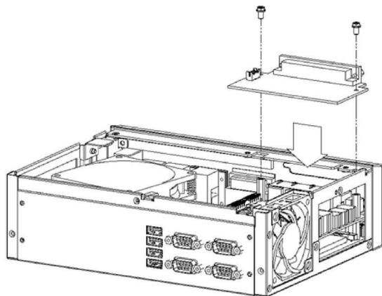
Figure 1: Installation Guide
