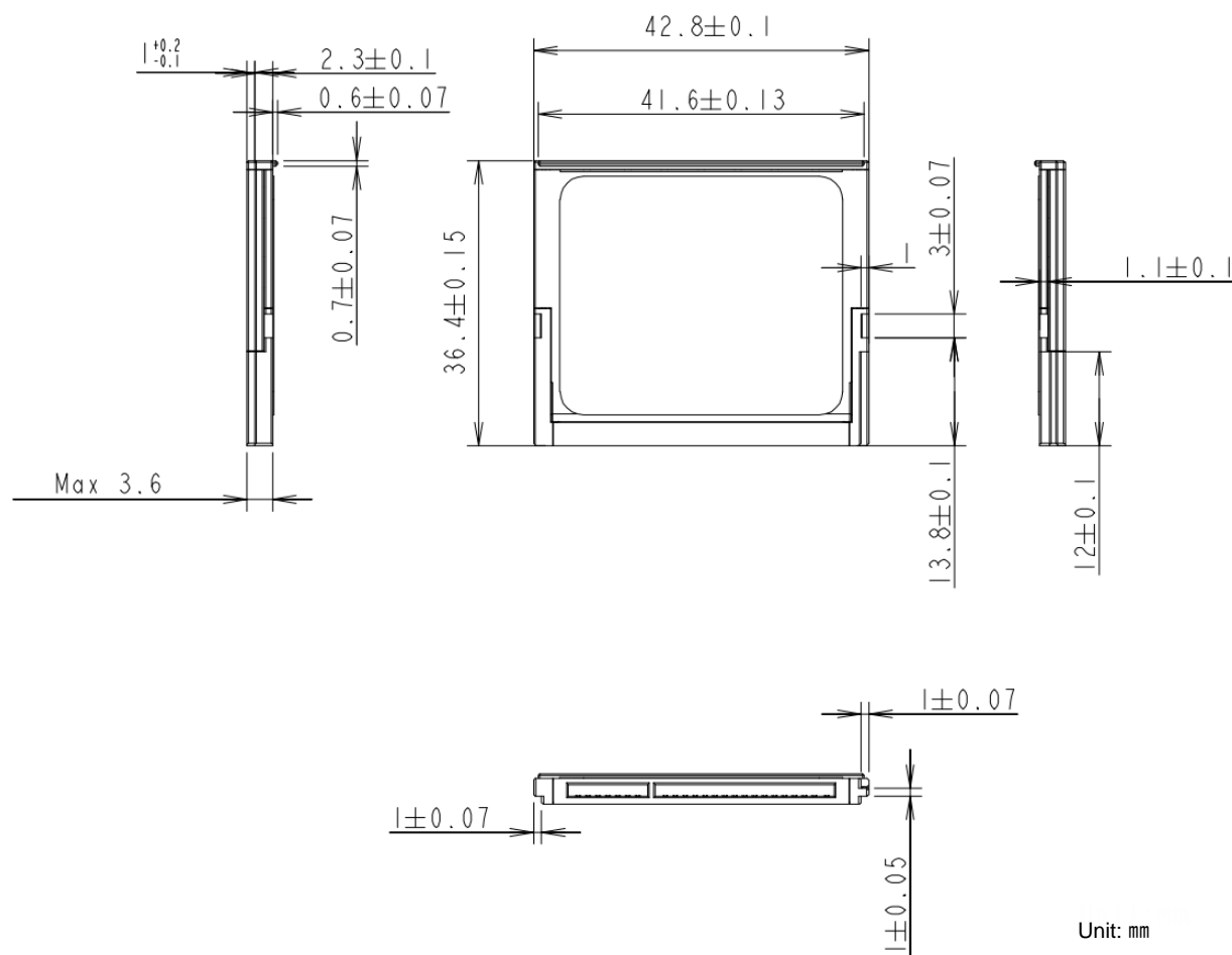
FIGURE 7-1 Physical dimension
