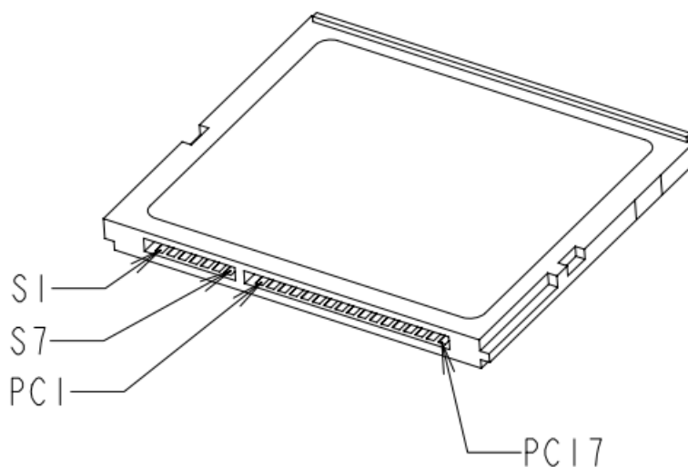
Figure 2-1 Pin Assignment
