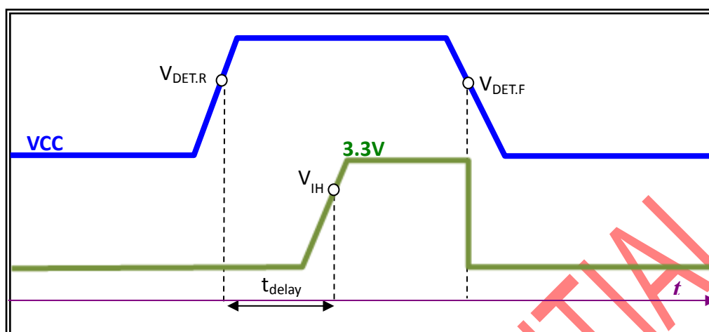
Figure 2 Power On Reset
