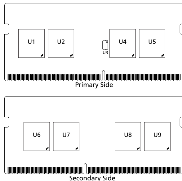
Figure 1: 260-Pin SODIMM
