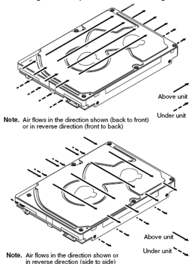
Figure 13. Air flow
