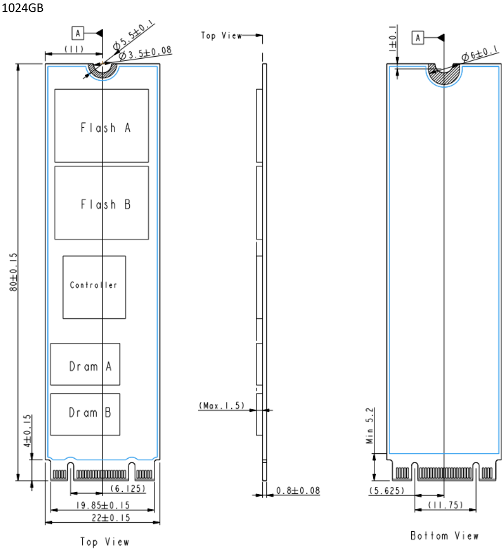
Dimension: 80.0 mm x 22.0 mm x 2.3 mm (L x W x H)
