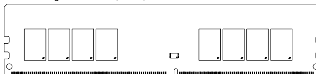
Figure 1: 288-Pin UDIMM (MO-309, R/C-B1)
