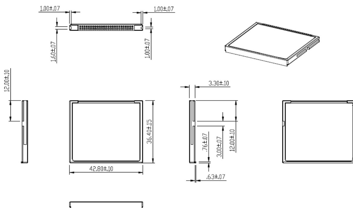
Figure 7-1 Physical Dimensions
