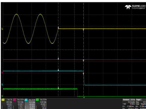
Figure 5: DS3000TE-3 Hold-up Time – V_{in} = 180\text{Vac} / 63\text{Hz} / 0^\circ Full Load: I_o = 223\text{A} , I_{SB} = 4.5\text{A} Ch 1: AC Mains Ch 2: V_{SB} Ch 3: V_o Ch 4: PWOK
