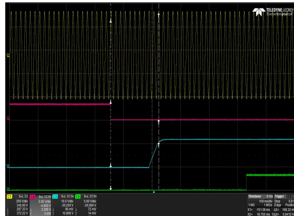
Figure 4: DS3000TE-3 Turn-on delay via PSOn – V_{in} = 264\text{Vac} Full Load: I_o = 248\text{A} , I_{SB} = 4.5\text{A} Ch 1: AC Mains Ch 2: PSOn Ch 3: V_o Ch 4: PWOK
