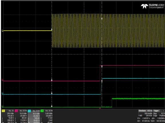
Figure 1: DS3000TE-3 Turn-on delay via AC mains – V_{in} = 180\text{Vac} Full Load: I_o = 223\text{A} , I_{SB} = 4.5\text{A} Ch 1: AC Mains Ch 2: V_{SB} Ch 3: V_o Ch 4: PWOK
