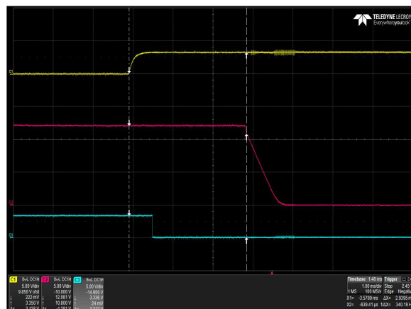
Figure 12: DS3000TE-3 Turn Off Characteristic via PSN – V_{in} = 264\text{Vac} Full Load: I_O = 248\text{A} , I_{SB} = 4.5\text{A} Ch 1: PSN Ch 2: V_O Ch 3: PWOK
