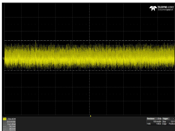
Figure 9: DS3000TE-3 Ripple and Noise Measurement – V_{in} = 180\text{Vac} Full Load: I_O = 223\text{A} , I_{SB} = 4.5\text{A} Ch 1: V_O
