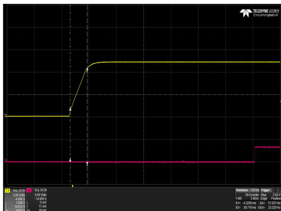
Figure 7: DS3000TE-3 Output Voltage Startup – V_{in} = 180\text{Vac} Full Load: I_O = 223\text{A} , I_{SB} = 4.5\text{A} Ch 1: V_O Ch 2: PWOK
