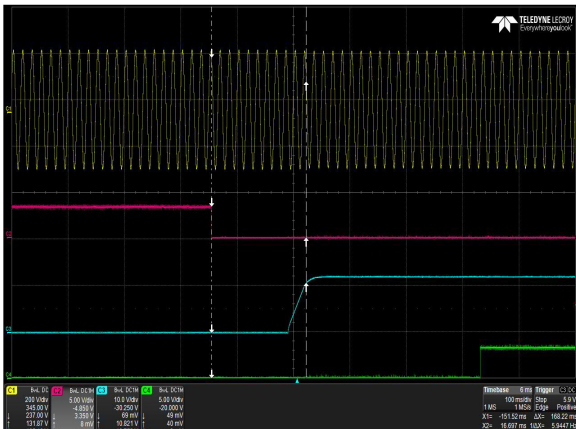
Figure 3: DS3000TE-3 Turn-on delay via PSOn – V_{in} = 180\text{Vac} Full Load: I_o = 223\text{A} , I_{SB} = 4.5\text{A} Ch 1: AC Mains Ch 2: PSOn Ch 3: V_o Ch 4: PWOK
