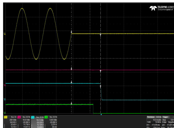
Figure 6: DS3000TE-3 Hold-up Time – V_{in} = 264\text{Vac} / 47\text{Hz} / 0^\circ Full Load: I_o = 248\text{A} , I_{SB} = 4.5\text{A} Ch 1: AC Mains Ch 2: V_{SB} Ch 3: V_o Ch 4: PWOK
