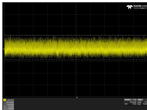
Figure 10: DS3000TE-3 Ripple and Noise Measurement – V_{in} = 264\text{Vac} Full Load: I_O = 248\text{A} , I_{SB} = 4.5\text{A} Ch 1: V_O
