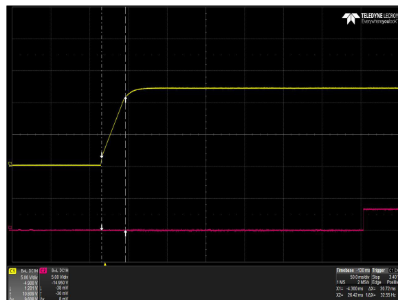
Figure 8: DS3000TE-3 Output Voltage Startup – V_{in} = 264\text{Vac} Full Load: I_O = 248\text{A} , I_{SB} = 4.5\text{A} Ch 1: V_O Ch 2: PWOK
