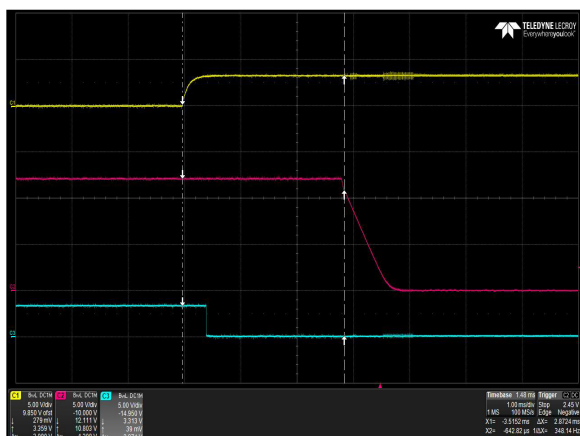
Figure 11: DS3000TE-3 Turn Off Characteristic via PSN – V_{in} = 180\text{Vac} Full Load: I_O = 223\text{A} , I_{SB} = 4.5\text{A} Ch 1: PSN Ch 2: V_O Ch 3: PWOK
