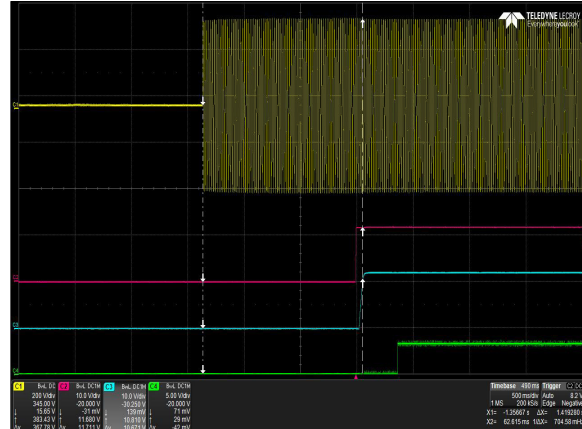
Figure 2: DS3000TE-3 Turn-on delay via AC mains – V_{in} = 264\text{Vac} Full Load: I_o = 248\text{A} , I_{SB} = 4.5\text{A} Ch 1: AC Mains Ch 2: V_{SB} Ch 3: V_o Ch 4: PWOK
