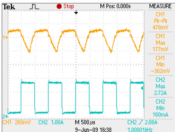
Figure 11: ADNB027-15-1PM-C Transient Response Vin = 230Vac Load: Io = FULL/MIN LOAD, 90%DUTY/1KHZ Ch 1: Vo Ch 2: Iout
