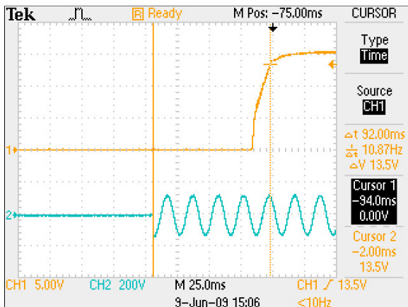
Figure 9: ADNB027-15-1PM-C Turn-on delay – Vin= 90Vac Load: Io = 2.7A Ta = 25 °C Ch 1: Vo Ch2:AC Mains
