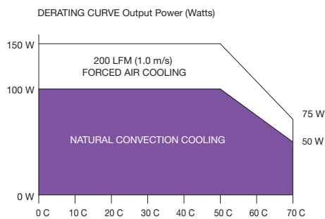
Figure 1: Derating Curve
