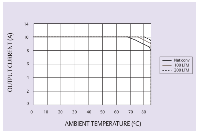
Figure 2 - Safe Operating Area V in = 12 V, V REF = 1.25 V, I out = 10 A (See Note A)
