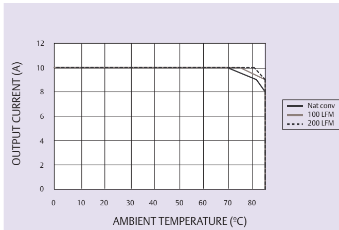
Figure 1 - Safe Operating Area V in = 5.0 V, V REF = 1.25 V, I out = 10 A (See Note A)
