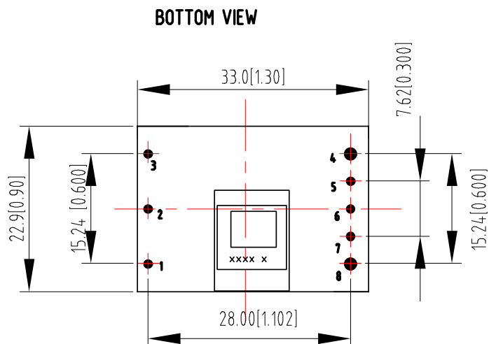
Model: AVD50B-48S05B-6L
