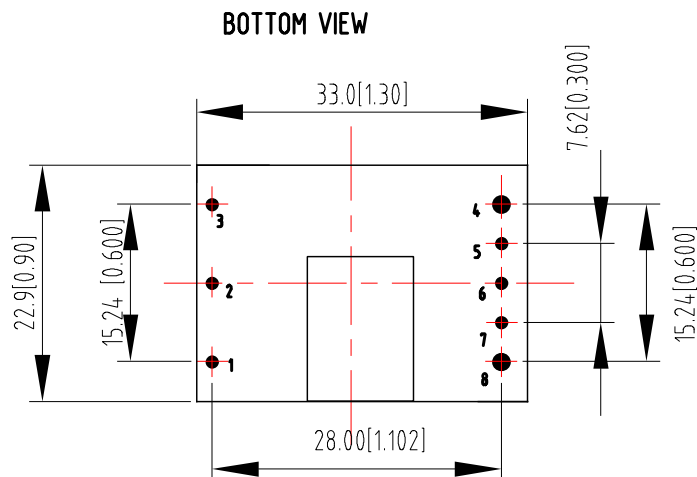
Model: AVD50B-48S05-6L
