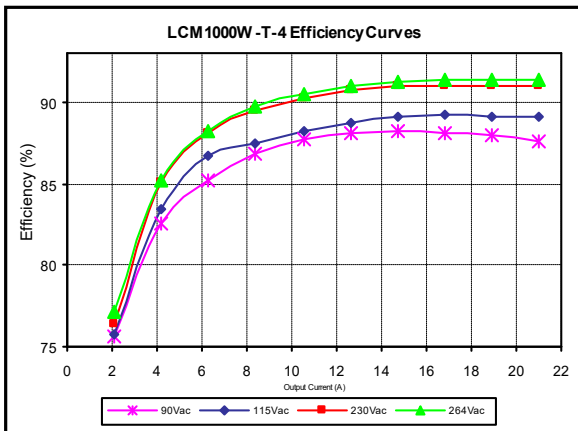
Figure 54: LCM1000W-T-4 Efficiency Curves @ 25 °C
