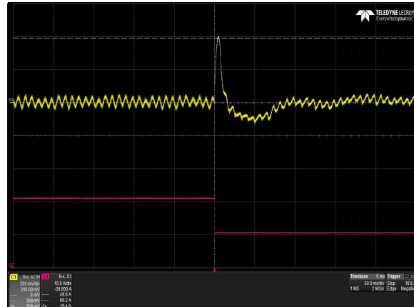
Figure 53: LCM1000W-T-4 Transient Response – V_O Deviation (high to low) 100% to 50% load change, 1A/uS slew rate, V_{IN} = 90\text{Vac} Ch 1: V_O Ch 2: I_O
