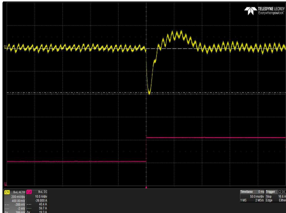
Figure 52: LCM1000W-T-4 Transient Response – V_O Deviation (low to high) 50% to 100% load change, 1A/uS slew rate, V_{IN} = 90\text{Vac} Ch 1: V_O Ch 2: I_O
