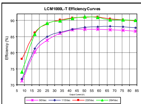
Figure 10: LCM1000L-T Efficiency Curves @ 25 °C
