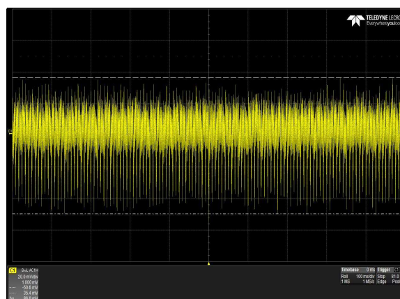
Figure 11: LCM1000L-T Ripple and Noise Measurement – V_{IN} = 90\text{Vac} Full Load: I_O = 83.3\text{A} (12V)
