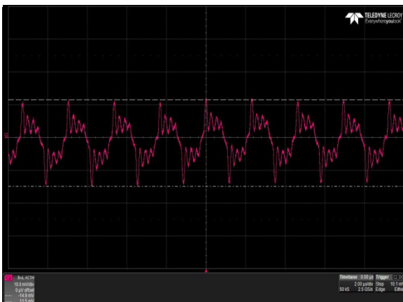
Figure 5: AIQ02R300-L Ripple and Noise Measurement - V_{in} = 390V_{dc} No Load: I_o = 0A , Ch 2: V_o
