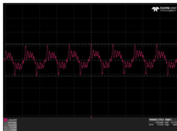
Figure 6: AIQ02R300-L Ripple and Noise Measurement - V_{in} = 390V_{dc} Full Load: I_o = 2.32A , Ch 2: V_o
