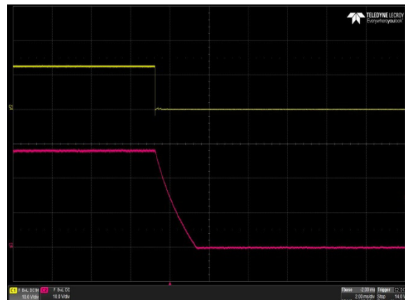
Figure 4: AIQ02R300-L Turn-off Characteristic via Enable - V_{in} = 390V_{dc} Full Load: I_o = 2.32A , Ch 1: Enable Ch 2: V_o
