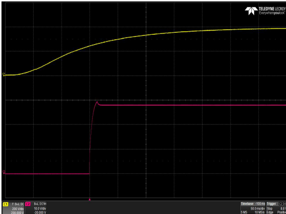
Figure 1: AIQ02R300-L Turn-on Characteristic via DC mains - V_{in} = 390V_{dc} Full Load: I_o = 2.32A , Ch 1: DC Mains Ch 2: V_o
