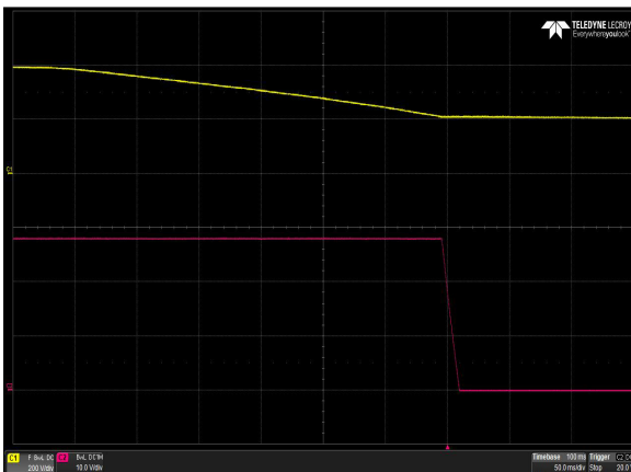
Figure 3: AIQ02R300-L Turn-off Characteristic via DC mains - V_{in} = 390V_{dc} Full Load: I_o = 2.32A , Ch 1: DC Mains Ch 2: V_o
