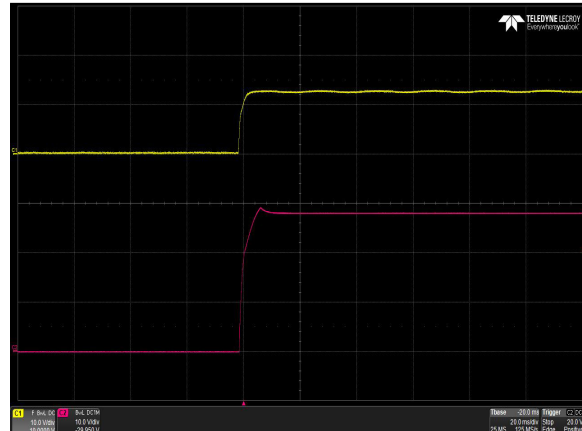
Figure 2: AIQ02R300-L Turn-on Characteristic via Enable V_{in} = 390V_{dc} Full Load: I_o = 2.32A , Ch 1: Enable Ch 2: V_o
