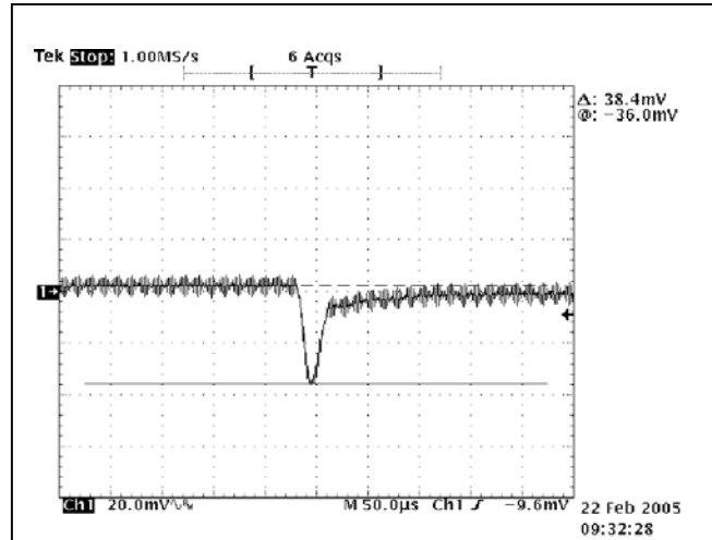
Figure 58. Transient Response at T_A = 25^\circ\text{C} , 1.2V OUT Deviation (Lo-Hi).
