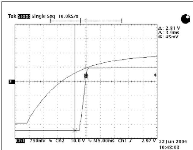
Figure 23. 3.3V OUT Startup Characteristic at V_{IN} = 48Vdc, I_O = Full Load, T_A = 25°C.
