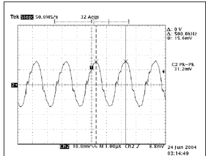
Figure 24. 3.3V OUT Ripple Waveform at V_{IN} = 48Vdc, I_O = Full Load, T_A = 25°C.
