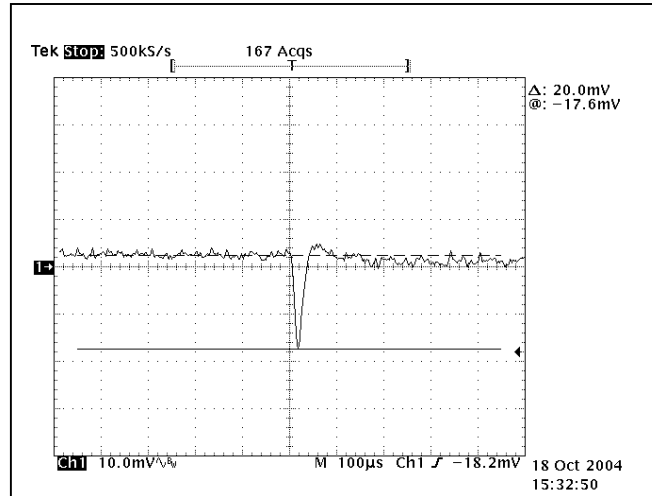
Figure 18. Transient Response at T_A = 25^\circ\text{C} , 5V_{OUT} Deviation (Lo-Hi).
