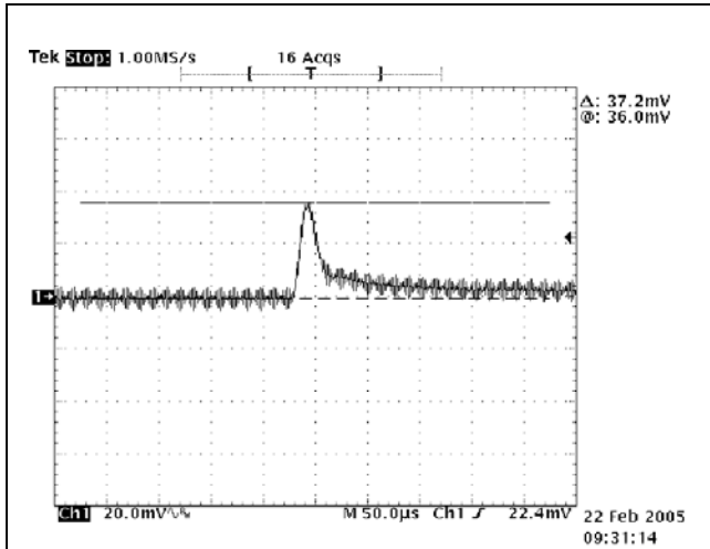
Figure 57. Transient Response at T_A = 25^\circ\text{C} , 1.2V OUT Deviation (Hi-Lo).
