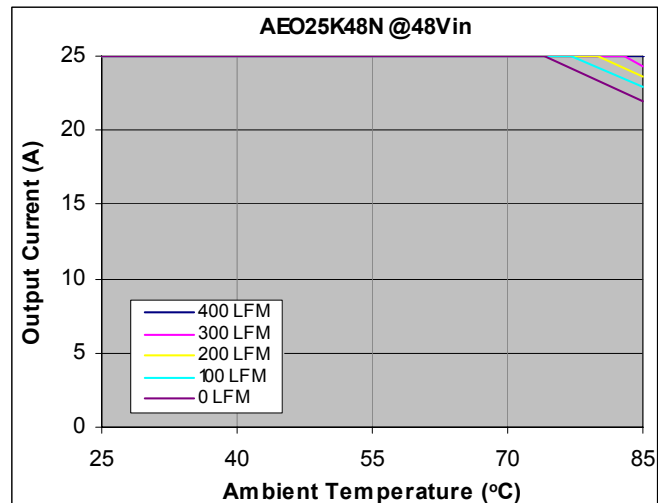
Figure 60. Output Current vs. Temperature for baseplate version at V_{IN} = 48\text{Vdc} , T_A = 25^\circ\text{C} .
