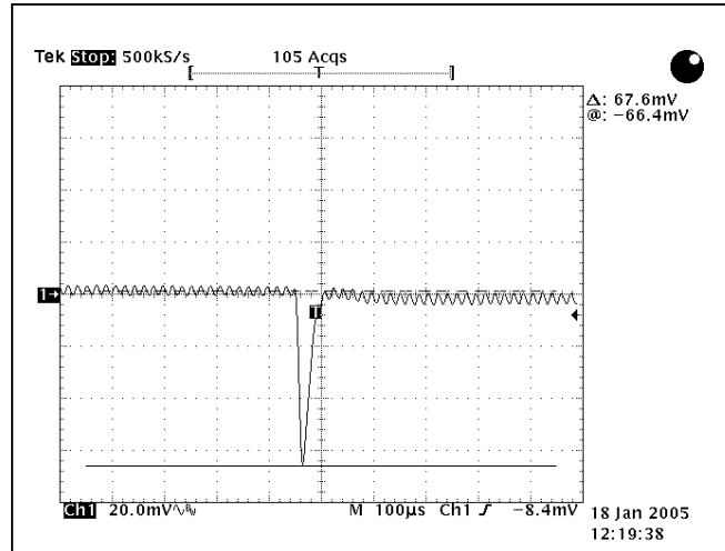
Figure 10. Transient Response at T_A = 25^\circ\text{C} , 12V OUT Deviation (Lo-Hi).
