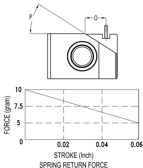
PLUNGER AND PLUNGER TIP SHOWN IN FULLY ACTIVATED POSITION
