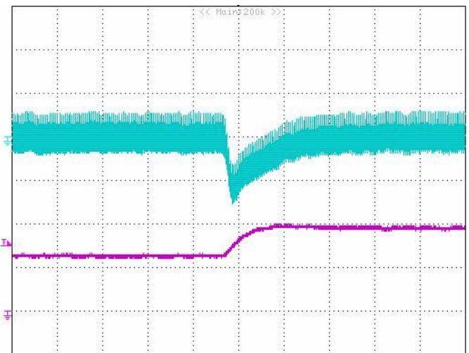
Figure 9: Output voltage response to step-change in load current (50%-75% of I_{o,max} ; di/dt = 1A/\mu s ). Load cap: 2310uF electrolytic capacitor. Top Trace: Vout (20mV/div, 100us/div), Bottom Trace: I_o (20A/div, 100us/div), Scope measurement should be made using a BNC cable (length shorter than 20 inches). Position the load between 51 mm to 76 mm (2 inches to 3 inches) from the module.
