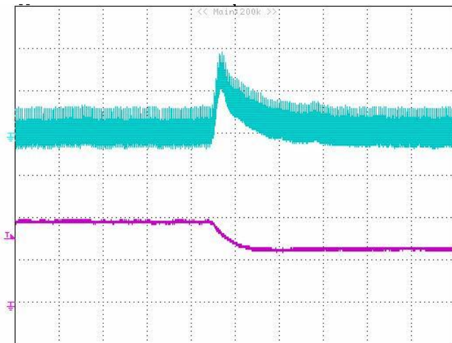
Figure 8: Output voltage response to step-change in load current (75%-50% of I_{o,max} ; di/dt = 1A/\mu s ). Load cap: 2310uF electrolytic capacitor. Top Trace: Vout (20mV/div, 100us/div), Bottom Trace: I_o (20A/div, 100us/div), Scope measurement should be made using a BNC cable (length shorter than 20 inches). Position the load between 51 mm to 76 mm (2 inches to 3 inches) from the module.
