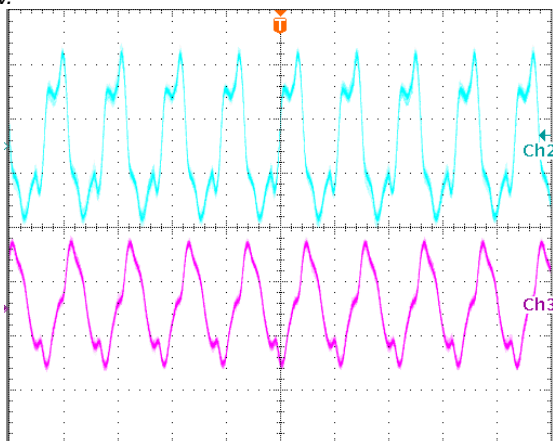
Output voltage ripple at nominal input voltage and max load current Top trace +15V, 10 mV/div, Bottom trace -15V, 20 mV/div, 2 \mu s/div. Load cap: 10 \mu F, tantalum capacitor and 1 \mu F ceramic capacitor. Bandwidth: 20 MHz.
