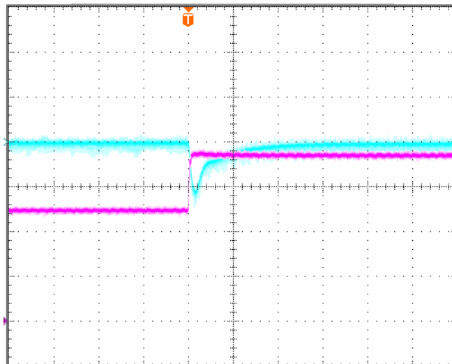
Figure 9: Output voltage response to step-change in load current (50%-75% of I_o , max; di/dt = 1A/\mu s ). Load cap: 400 \mu F , ceramic capacitor. Top Trace: Vout (100mV/div, 200us/div); Bottom Trace: output current (1.5A/div, 200us/div)
