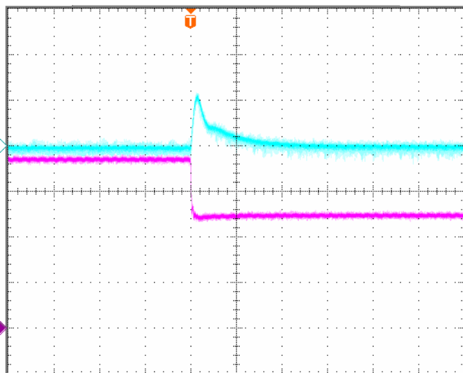
Figure 8: Output voltage response to step-change in load current (75%-50% of I_o , max; di/dt = 1A/\mu s ). Load cap: 400 \mu F , ceramic capacitor. Top Trace: Vout (100mV/div, 200us/div); Bottom Trace: output current (1.5A/div, 200us/div)
