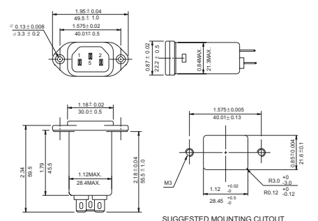
SUGGESTED MOUNTING CUTOUT
