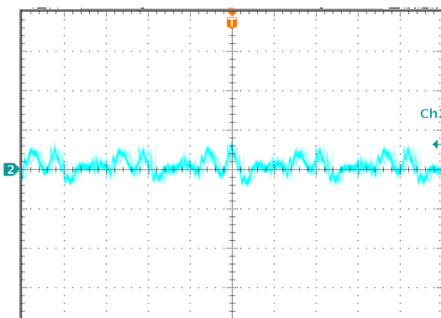
Figure 6: Output voltage ripple at V_{in}=72V and full load Trace: Vout: 10 mV/div, 2μs/div; Bandwidth: 20 MHz.
