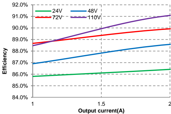
Figure 1: Efficiency vs. load current at 25°C.
