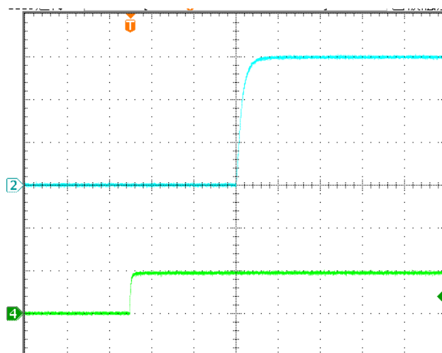
Figure 4: Turn-on transient at full load current (100ms/div). Top Trace: Vout, 8V/div; Bottom Trace: ON/OFF, 5V/div
