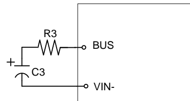
Figure 11 BUS pin circuit
