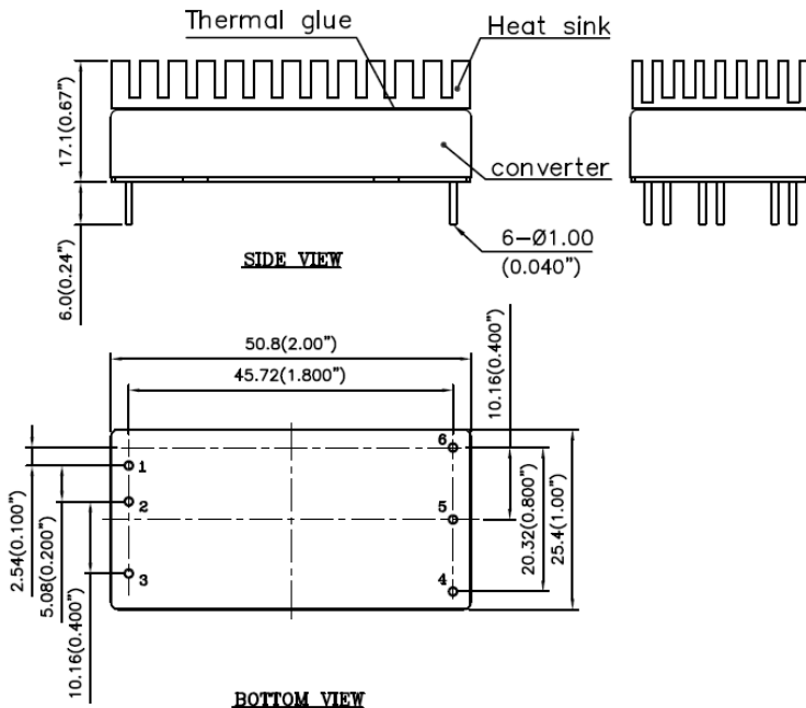
Mechanical Dimensions
