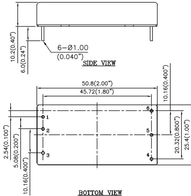
Mechanical Dimensions
