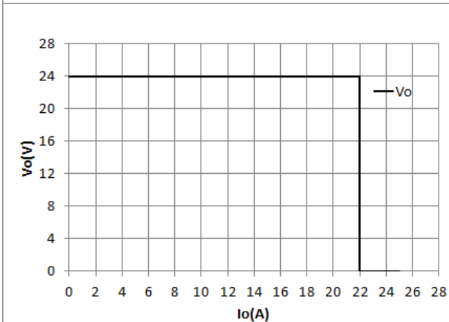
Figure 3: Output voltage vs. Output current @ V_{in}=110/220VAC
