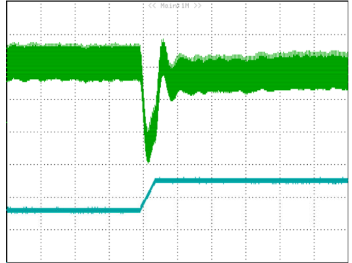
Figure 9: Output voltage response to step-change in load current (50%-75% of I_o max; di/dt = 0.1A/\mu s ). Load cap: 100uF Al-Electrolytic capacitor, 10uF tantalum capacitor and 1uF ceramic capacitor. Top Trace: Vout; 100mV/div; Bottom Trace: output current: 10A/div, Time: 200us/div
