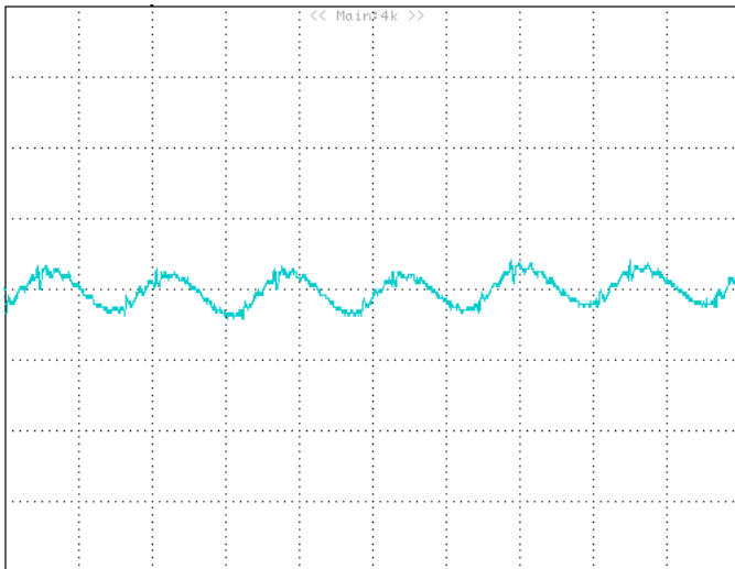
Figure 12: Input reflected ripple current, is, through a 12μH source inductor at nominal input voltage and rated load current (20 mA/div, 2μs/div).
