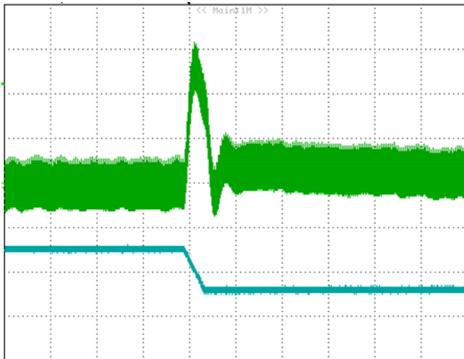
Figure 8: Output voltage response to step-change in load current (75%-50% of I_o max; di/dt = 0.1A/\mu s ). Load cap: 100uF Al-Electrolytic capacitor, 10uF tantalum capacitor and 1uF ceramic capacitor Top Trace: Vout; 100mV/div; Bottom Trace: output current: 10A/div, Time: 200us/div
