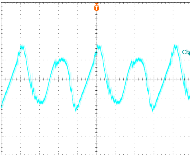
Figure 14: Output voltage ripple at nominal input voltage and rated load current ( I_o=33A ) (30 mV/div, 2μs/div) Load capacitance: 1μF ceramic capacitor and 10μF tantalum capacitor. Bandwidth: 20 MHz.
