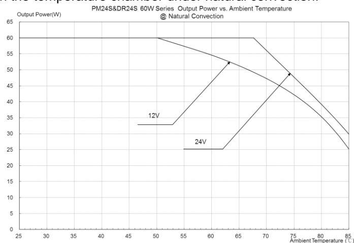
Figure1: PM24S12005&DR24S12005 60W series Output power vs Ambient temperature@Natural convection
