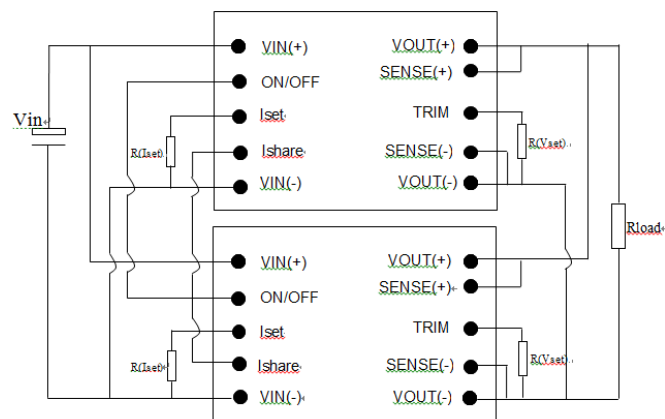
Figure 16: Parallel and current sharing configuration
