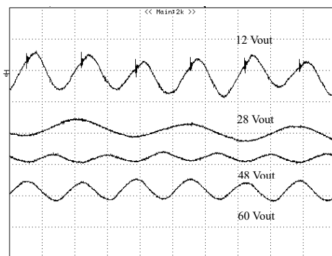
Figure 12: Input Terminal Ripple Current, i_c , at max output current and nominal input voltage(28V) with 12μH source impedance and 33μF electrolytic capacitor (50 mA/div, 2us/div).
