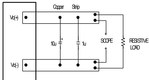
Figure 12: Output voltage noise and ripple measurement test setup
