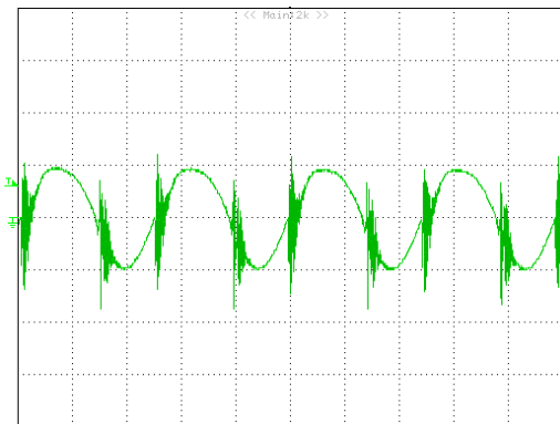
Figure 11: Input reflected ripple current, i_s , through a 12 \mu H source inductor at nominal input voltage and rated load current (20 mA/div, 2us/div)
