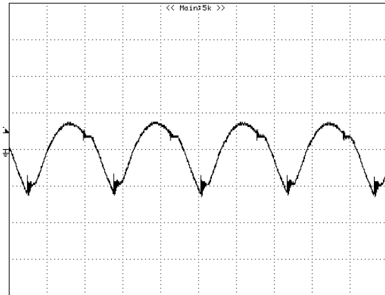
Figure 12: Output voltage ripple at nominal input voltage ( V_{in}=48V ) and rated load current ( I_o=4.2A ) (50 mV/div, 1μs/div). Load capacitance: 1μF ceramic capacitor and 10μF tantalum capacitor. Bandwidth: 20 MHz. Scope measurements should be made using a BNC cable (length shorter than 20 inches). Position the load between 51 mm to 76 mm (2 inches to 3 inches) from the module
