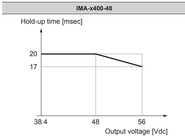
Fig. 15: Hold-up time versus output voltage 48 V
