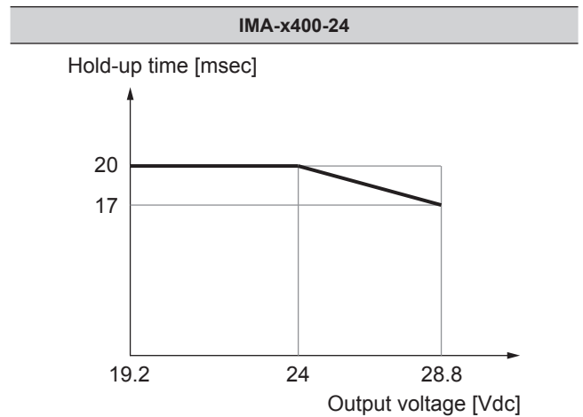
Fig. 14: Hold-up time versus output voltage 24 V
