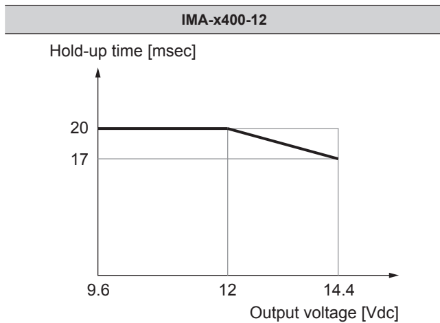
Fig. 13: Hold-up time versus output voltage 12 V
