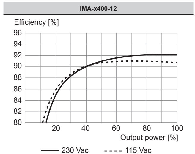
Fig. 16: Typical efficiency curves 12 V
