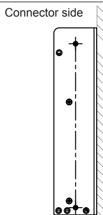
Fig. 2: Vertical mounting
