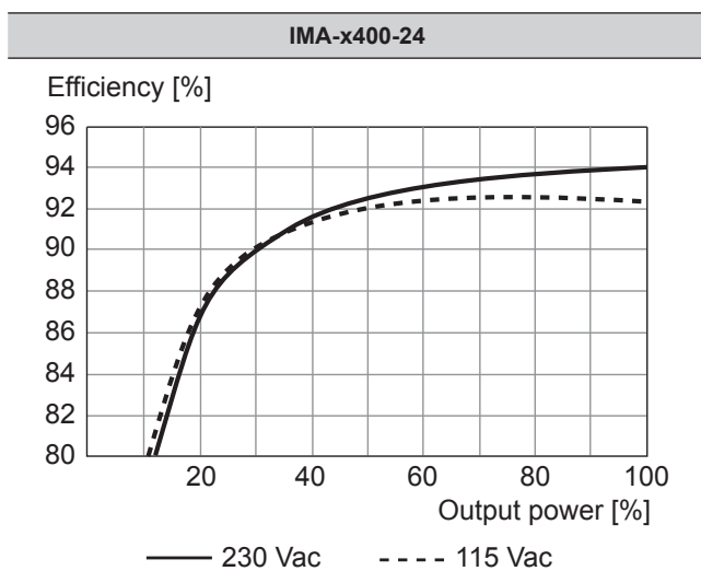
Fig. 17: Typical efficiency curves 24 V
