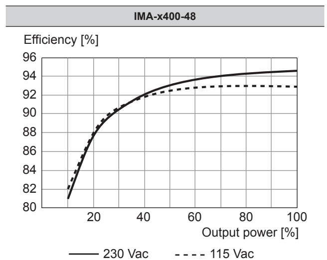
Fig. 18: Typical efficiency curves 48 V
