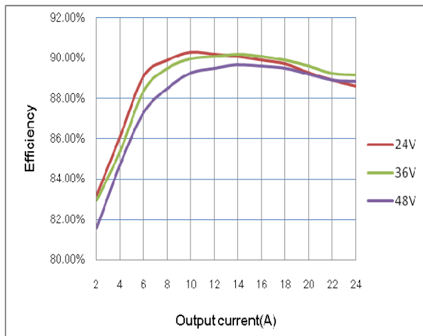
Figure 1: Efficiency vs. Output current @ V_{in}=24V, 36V, 48V (for A/B/C/D)
