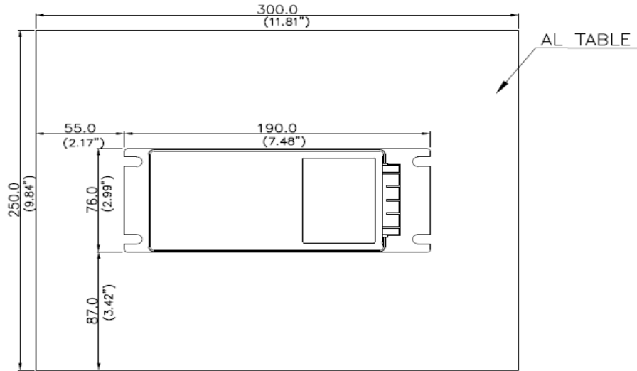
Figure 20: Thermal consideration
