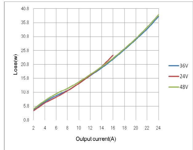
Figure 2: Loss vs. Output current @ V_{in}=24V, 36V, 48V (for A/B/C/D)
