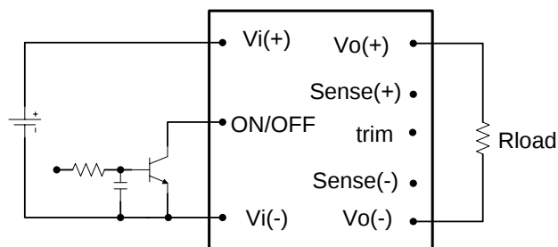
Figure 14: Remote on/off implementation
