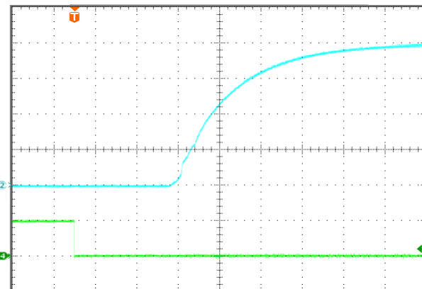
Figure 5: Turn-on transient at zero load current (10 ms/div). V_{in}=48V . Top Trace: V_{out} : 3.0V/div, Bottom Trace: ON/OFF input, 5V/div
