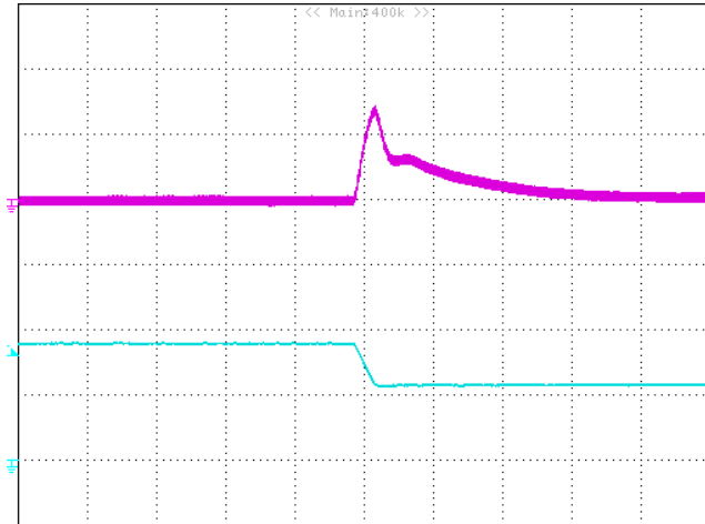
Figure 8: Output voltage response to step-change in load current (75%-50% of I_o , max; di/dt = 0.1A/\mu s , V_{in}=48V ). Load cap: 220 \mu F , electrolytic capacitor; 10 \mu F , tantalum capacitor and 1 \mu F ceramic capacitor. Top Trace: V_{out} (200mV/div, 200us/div); Bottom Trace: I_o (10A/div, 200us/div). Scope measurement should be made using a BNC cable (length shorter than 20 inches). Position the load between 51 mm to 76 mm (2 inches to 3 inches) from the module..
