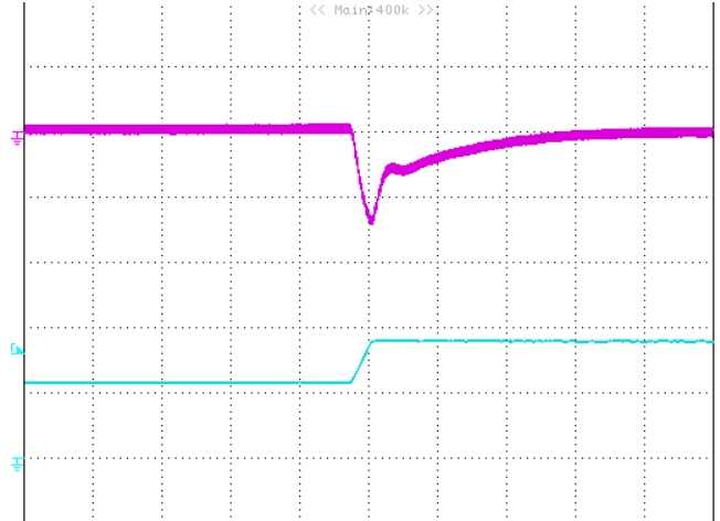
Figure 9: Output voltage response to step-change in load current (50%-75% of I_o , max; di/dt = 0.1A/\mu s , V_{in}=48V ). Load cap: 220 \mu F , electrolytic capacitor; 10 \mu F , tantalum capacitor and 1 \mu F ceramic capacitor. Top Trace: V_{out} (200mV/div, 200us/div); Bottom Trace: I_o (10A/div, 200us/div). Scope measurement should be made using a BNC cable (length shorter than 20 inches). Position the load between 51 mm to 76 mm (2 inches to 3 inches) from the module..
