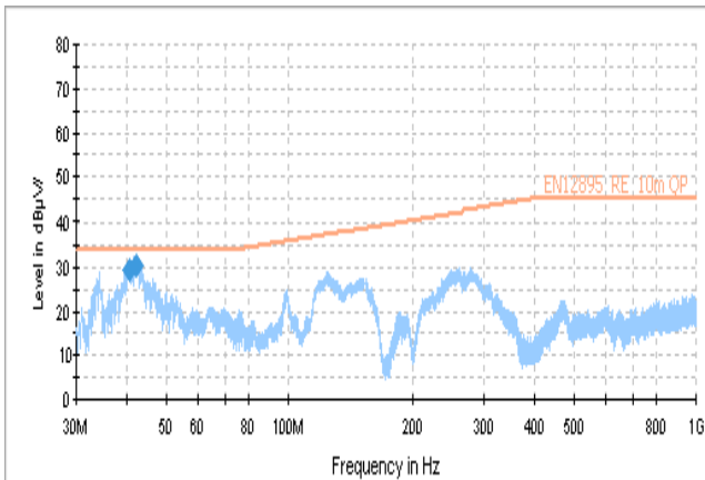
Figure 14: test result(Vertical)
