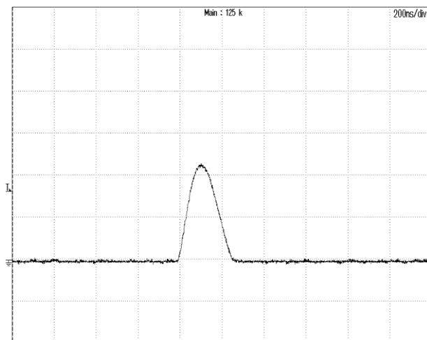
Figure 11: Inrush current @ Vin=72V CH1: I L , 2A/div, 200ns/div; Max current 4.3A, I 2t =1.5E-7 A 2 S
