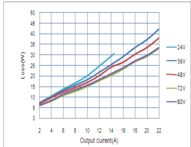
Figure 2: Loss vs. Output current @ Vin=24V,36V,48V, 72V, 80V
