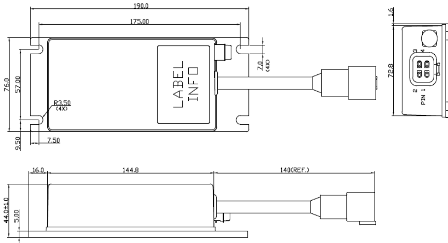
B70SR24125B
