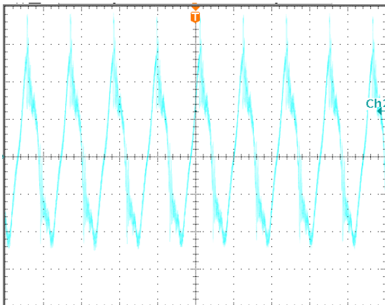
Output voltage ripple at nominal input voltage and max load current (5mV/div, 2μs/div) Load cap: 10μF, tantalum capacitor and 1μF ceramic capacitor. Bandwidth: 20 MHz.
