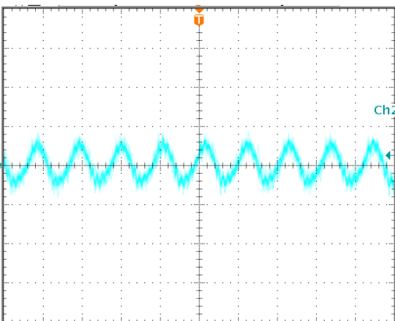
Output voltage ripple at nominal input voltage and max load current (4mV/div, 2us/div) Load cap: 10μF, tantalum capacitor and 1μF ceramic capacitor. Bandwidth: 20 MHz.
