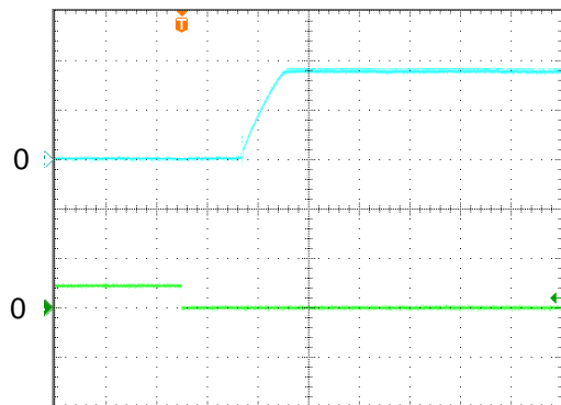
Figure 4: Turn-on transient at full rated load current (10 ms/div). V_{in}=48V . Top Trace: V_{out} , 1.0V/div; Bottom Trace: ON/OFF input, 5V/div
