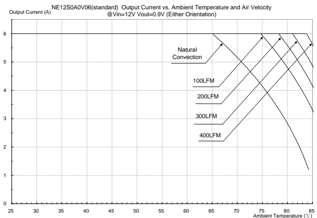
Figure 27: Output current vs. ambient temperature and air velocity @Vin=12V, Vout=0.9V (Either Orientation)
