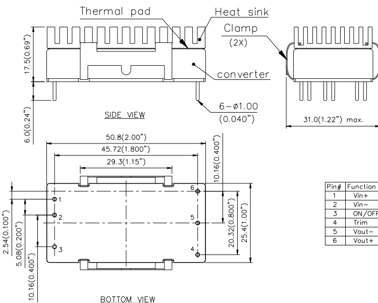
Mechanical Dimensions
